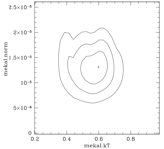
FIG. 5.— kT/\text{normalization} confidence contours (1, 2, 3 \sigma for two parameters) for the MEKAL thermal component in the power-law plus thermal component fit. The temperature ( kT ) of the thermal component is in keV. The normalization (mekal.norm) is in units of 10^{-14}/4\pi D^2 (emission measure). The sharp edges are an artifact of the relatively small number of points used to derive these contours.
