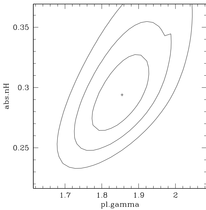
FIG. 4.— \Gamma/N_H confidence contours (1, 2, 3 \sigma for two parameters) for the absorbed power-law component in the power-law plus thermal component fit. N_H is in units of 10^{22}\text{cm}^{-2} .
